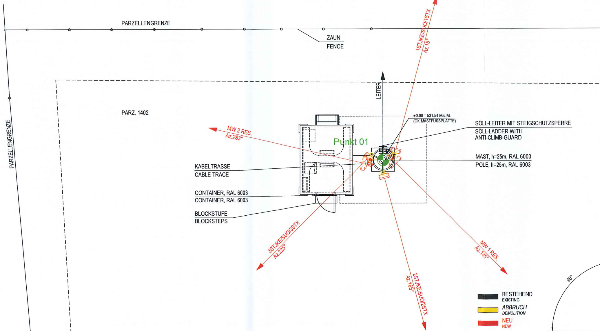
GRUNDRISS EQUIPMENT 1:50 ROOM LAYOUT 1:50 0 0.5m 2.5m
